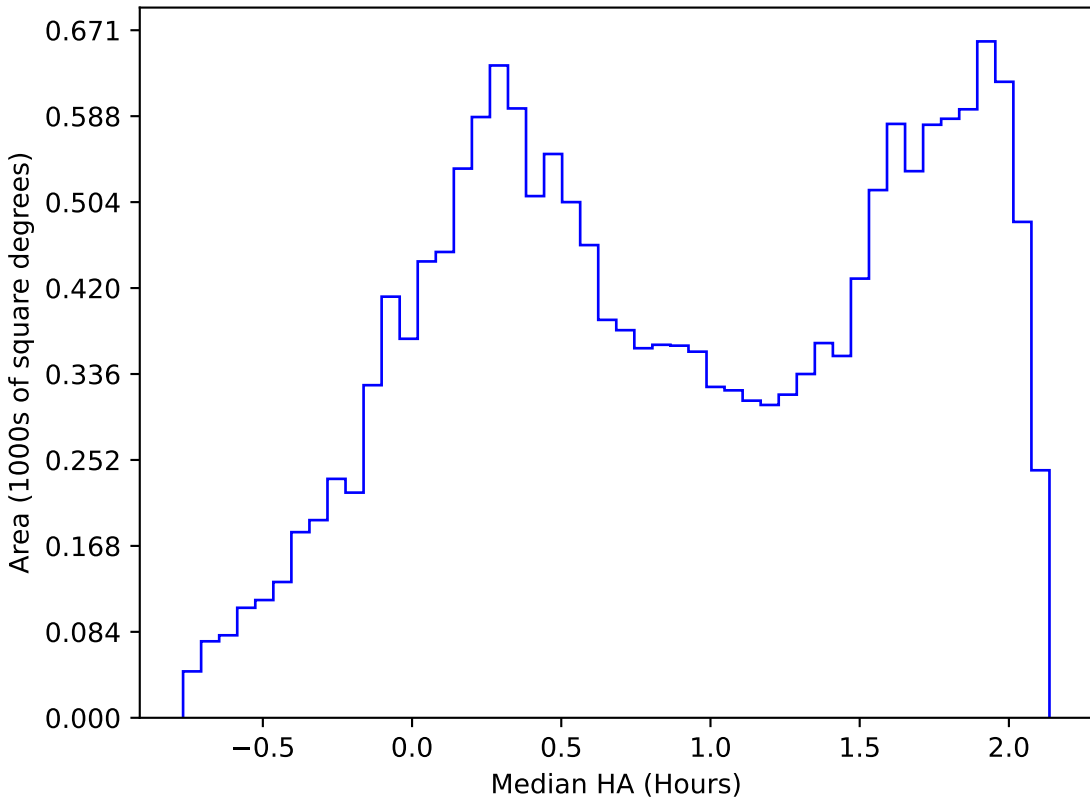
too_10_4v3.4_10yrs WFD r band: Median HA
