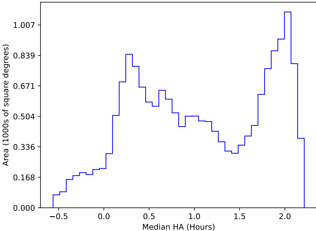
too_10_4v3.4_10yrs WFD i band: Median HA
