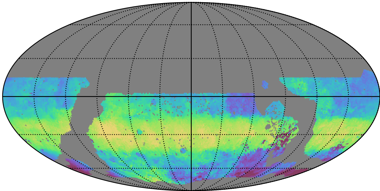
too_10_4v3.4_10yrs WFD g band: Median HA
