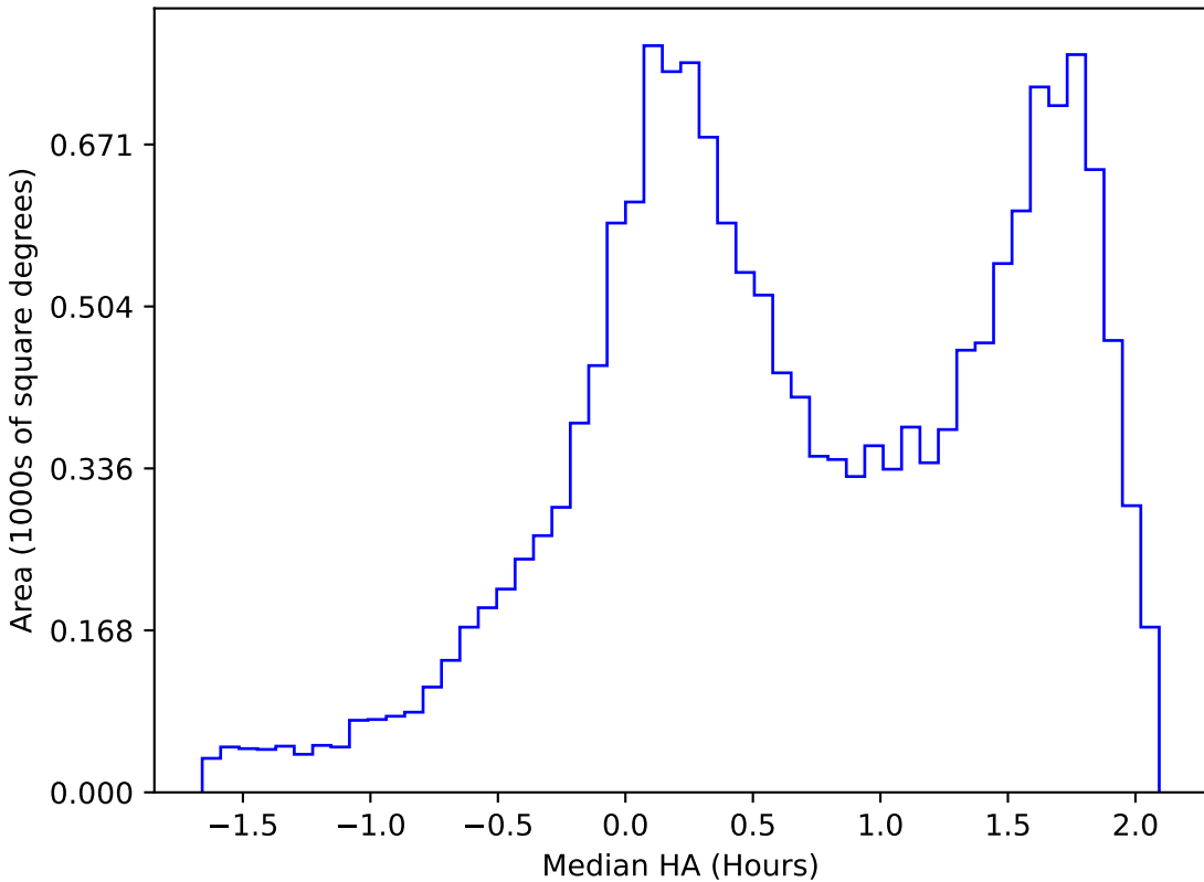
too_10_4v3.4_10yrs WFD g band: Median HA
