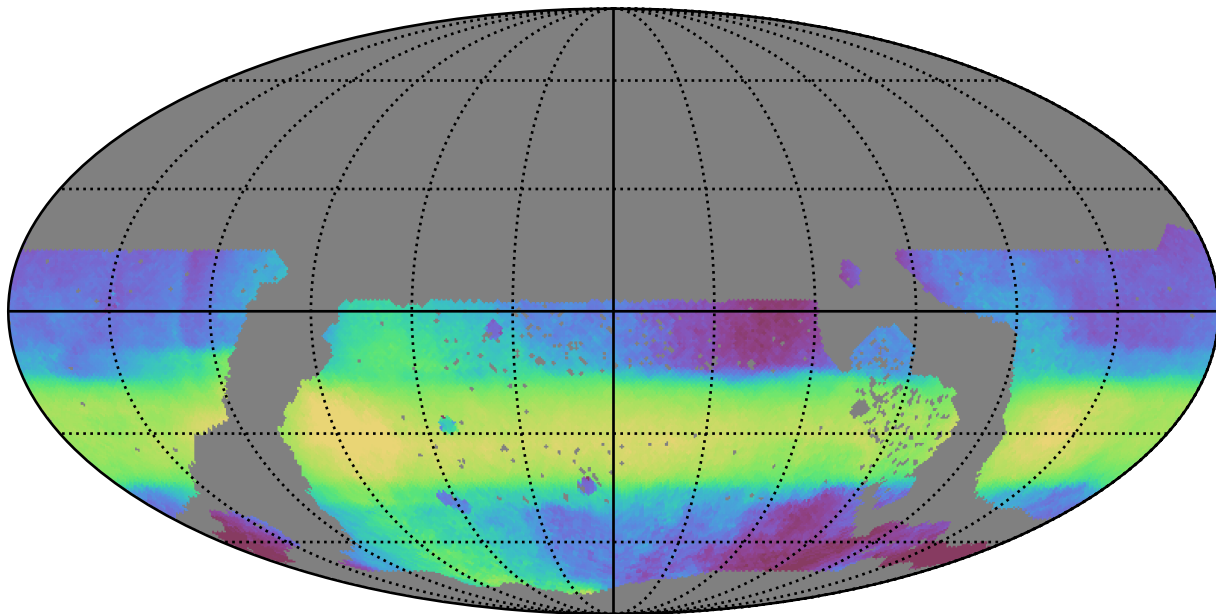
too_10_4v3.4_10yrs WFD all bands: Median HA
