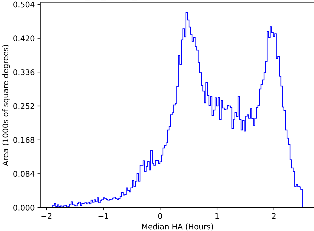
too_10_4v3.4_10yrs All sky z band: Median HA
