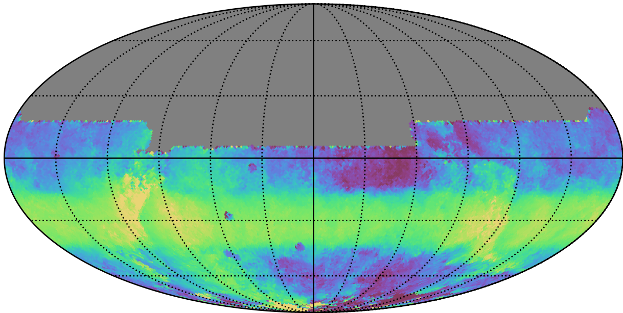
too_10_4v3.4_10yrs All sky y band: Median HA
