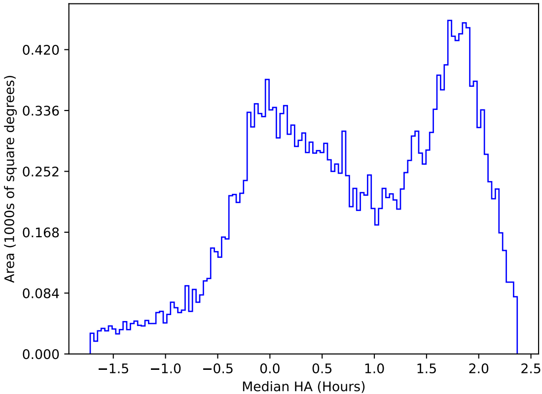
too_10_4v3.4_10yrs All sky u band: Median HA
