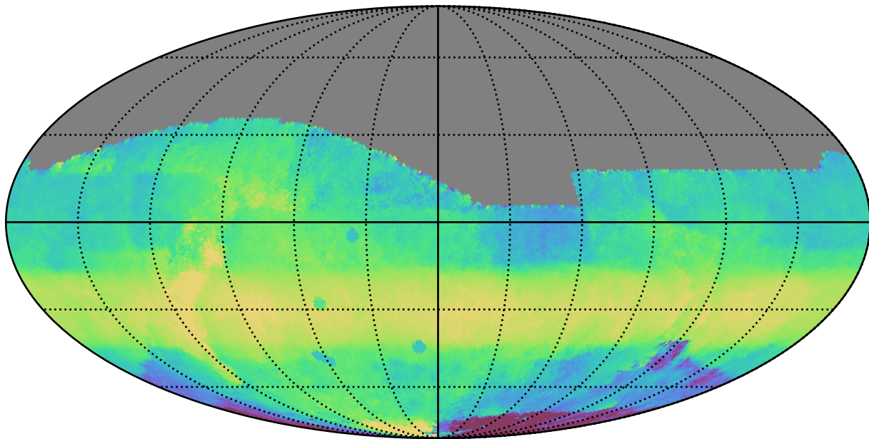
too_10_4v3.4_10yrs All sky i band: Median HA
