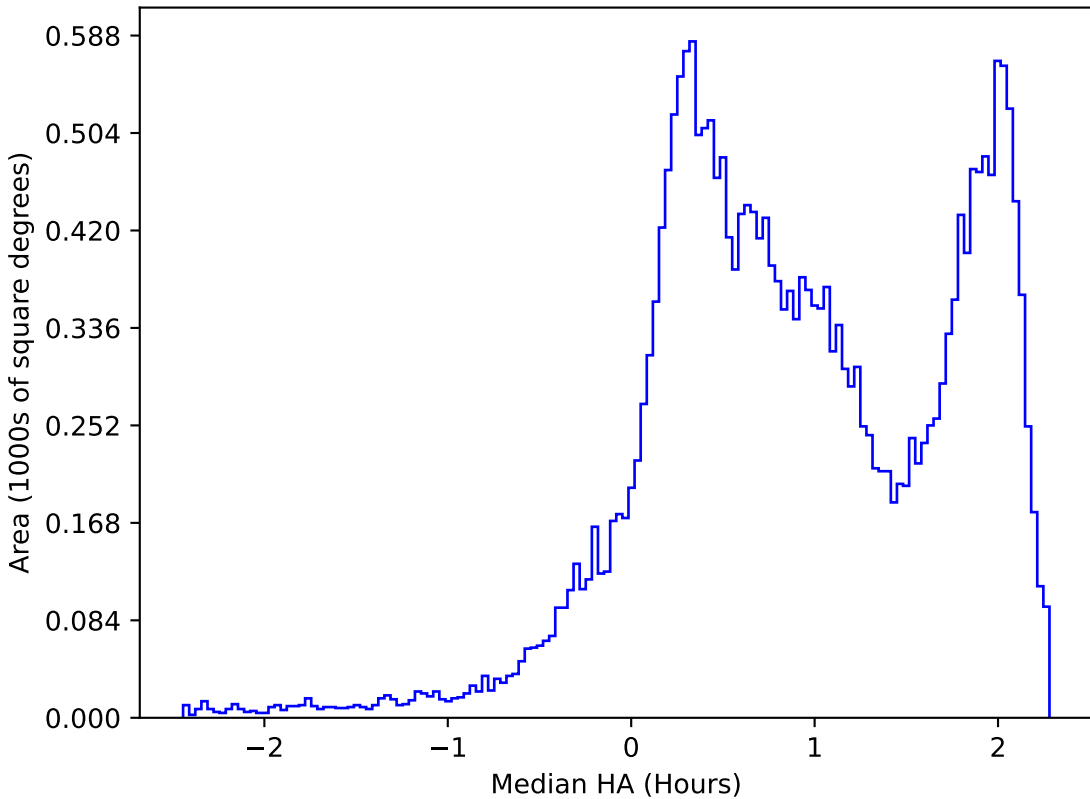
too_10_4v3.4_10yrs All sky i band: Median HA
