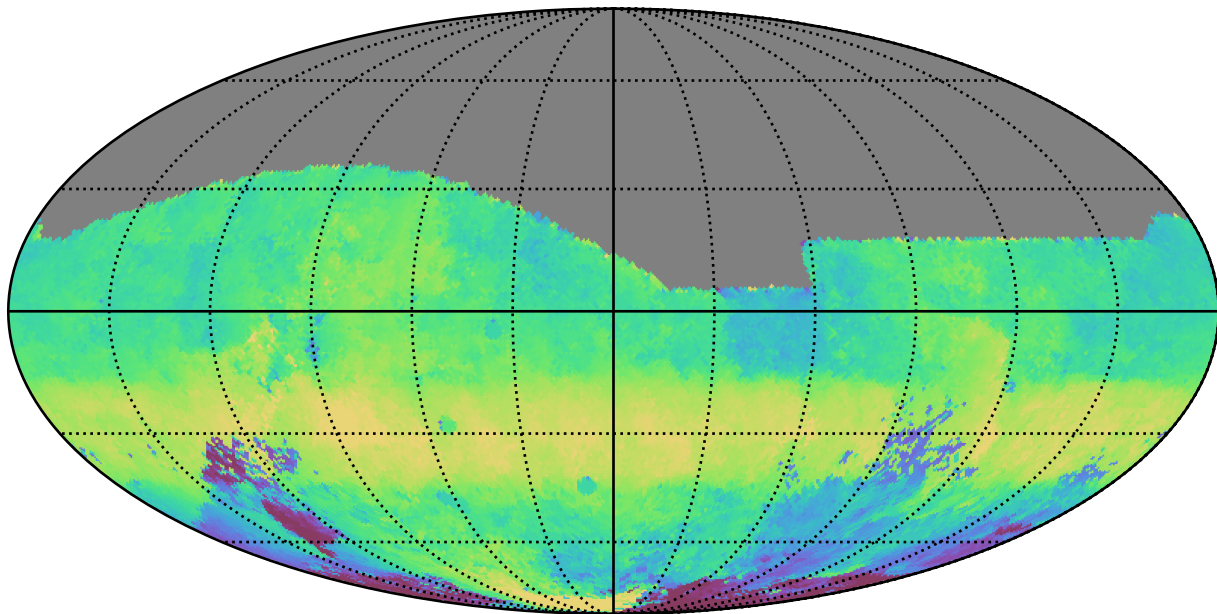
too_10_4v3.4_10yrs All sky g band: Median HA
