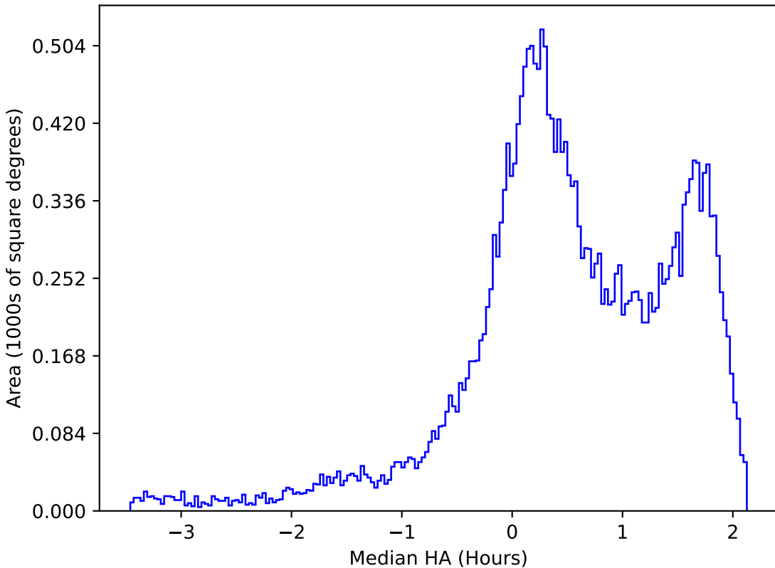
too_10_4v3.4_10yrs All sky g band: Median HA
