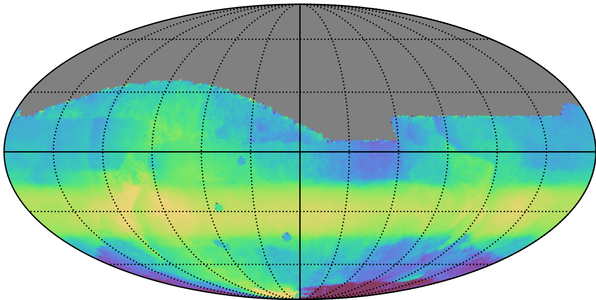
too_10_4v3.4_10yrs All sky all bands: Median HA
