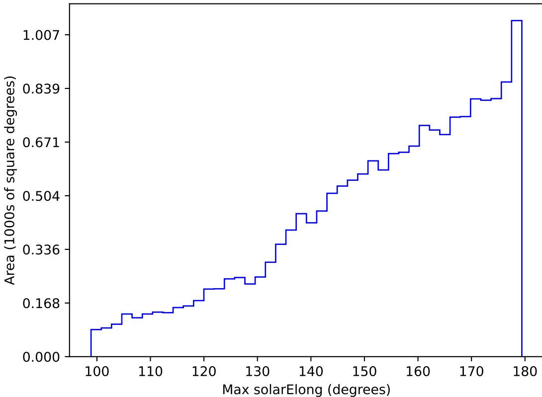
too_10_4v3.4_10yrs WFD z band: Max solarElong
