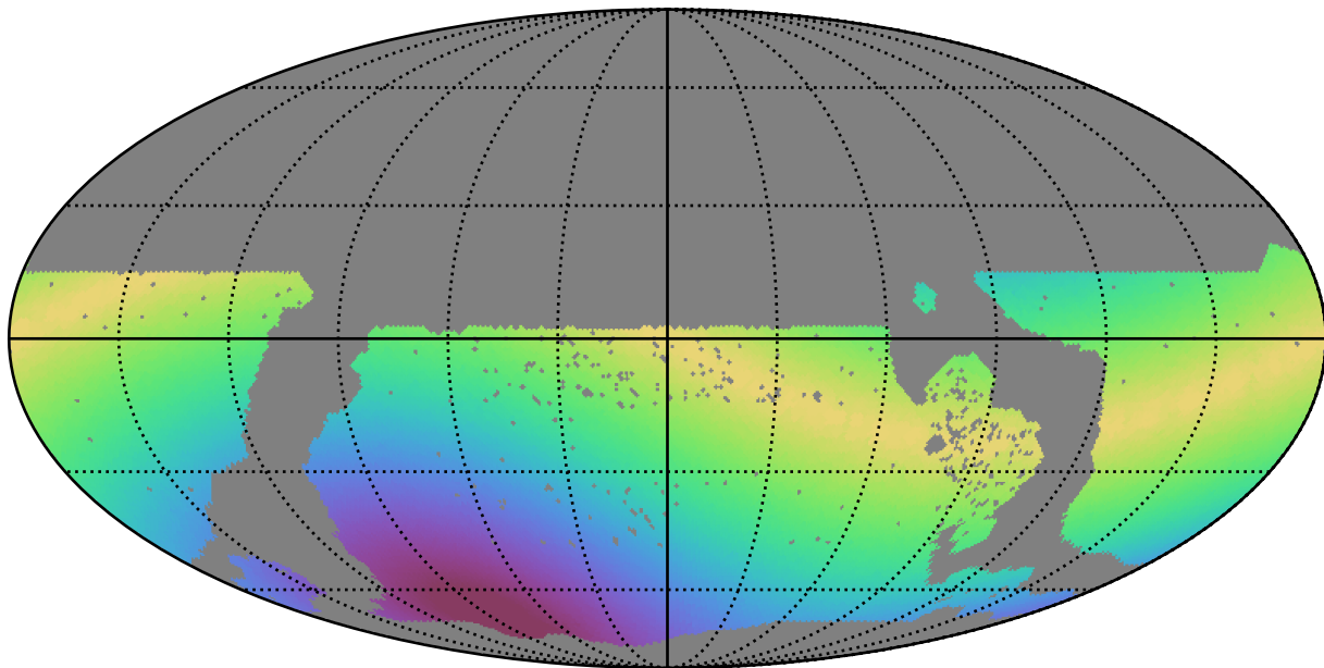
too_10_4v3.4_10yrs WFD y band: Max solarElong
