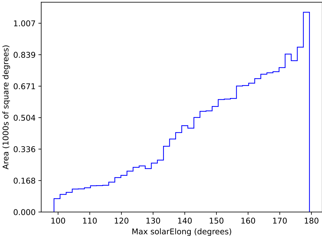
too_10_4v3.4_10yrs WFD r band: Max solarElong
