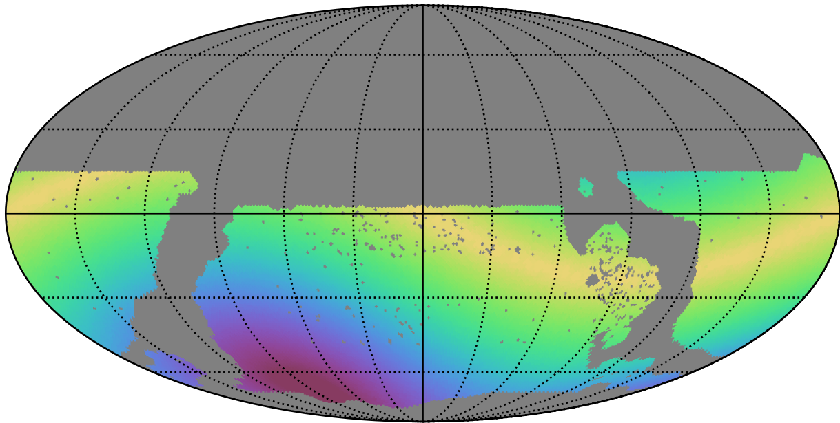
too_10_4v3.4_10yrs WFD i band: Max solarElong
