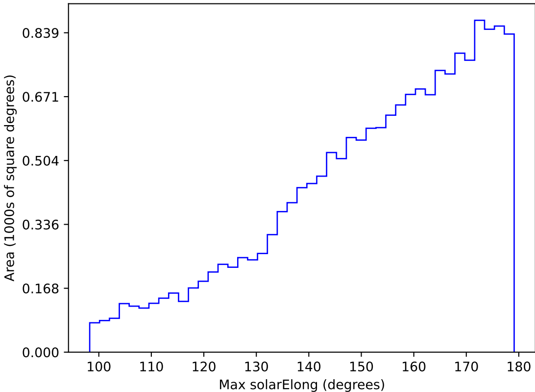
too_10_4v3.4_10yrs WFD g band: Max solarElong
