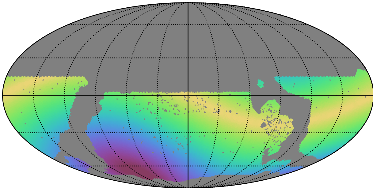
too_10_4v3.4_10yrs WFD all bands: Max solarElong
