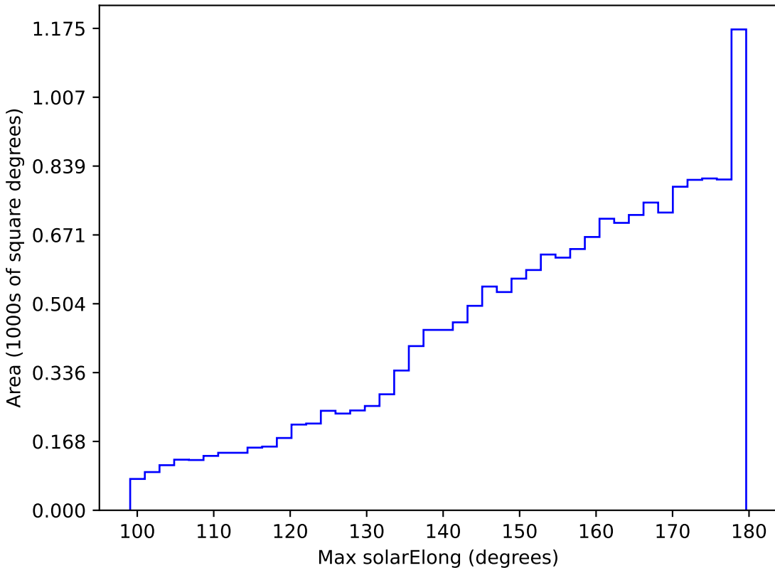
too_10_4v3.4_10yrs WFD all bands: Max solarElong
