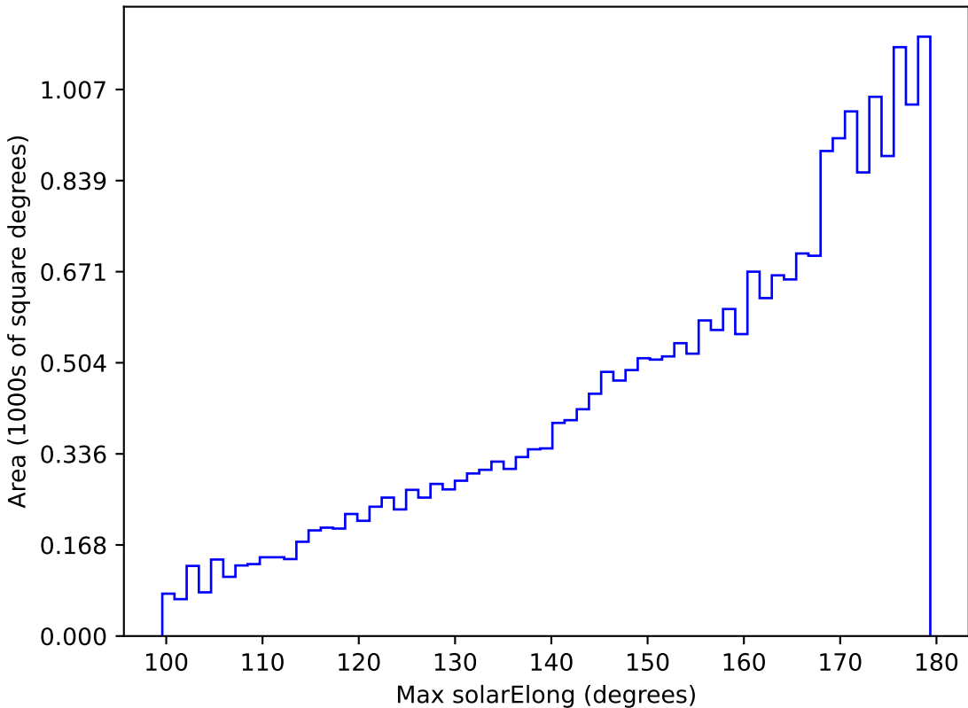
too_10_4v3.4_10yrs All sky z band: Max solarElong
