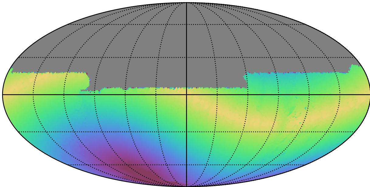
too_10_4v3.4_10yrs All sky u band: Max solarElong
