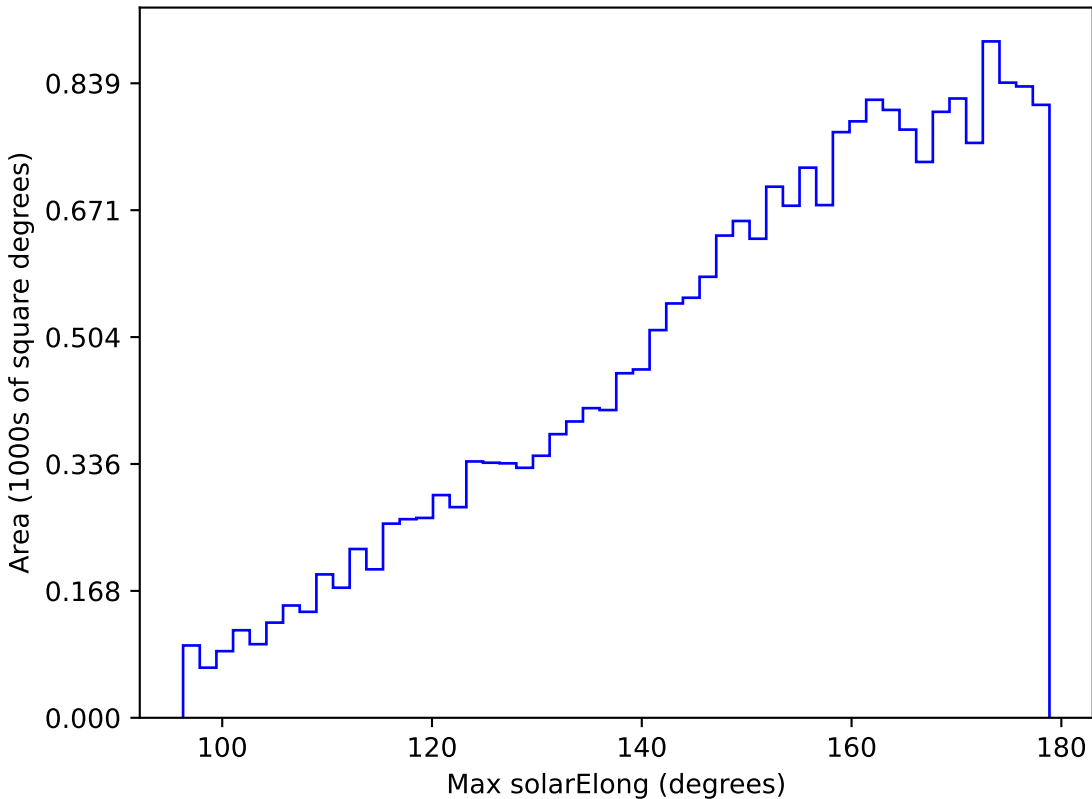
too_10_4v3.4_10yrs All sky u band: Max solarElong
