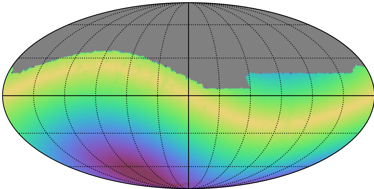
too_10_4v3.4_10yrs All sky r band: Max solarElong
