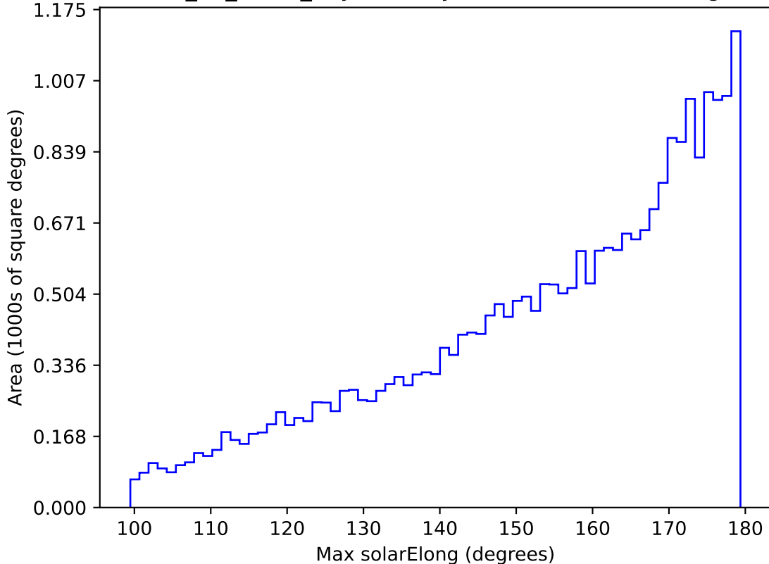
too_10_4v3.4_10yrs All sky r band: Max solarElong
