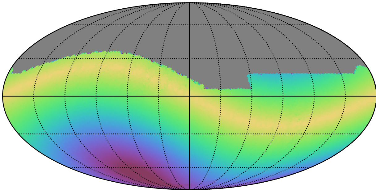
too_10_4v3.4_10yrs All sky i band: Max solarElong
