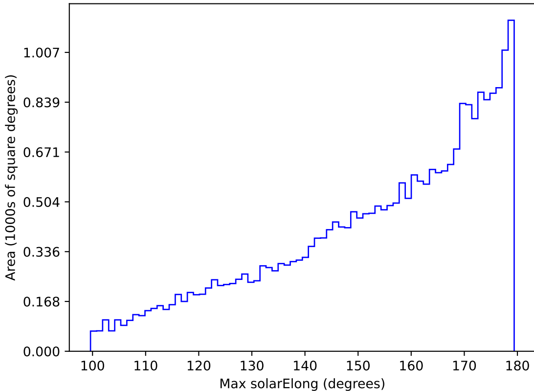
too_10_4v3.4_10yrs All sky i band: Max solarElong
