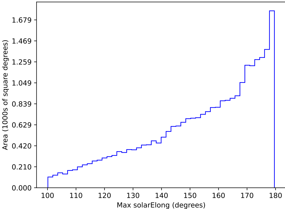
too_10_4v3.4_10yrs All sky all bands: Max solarElong
