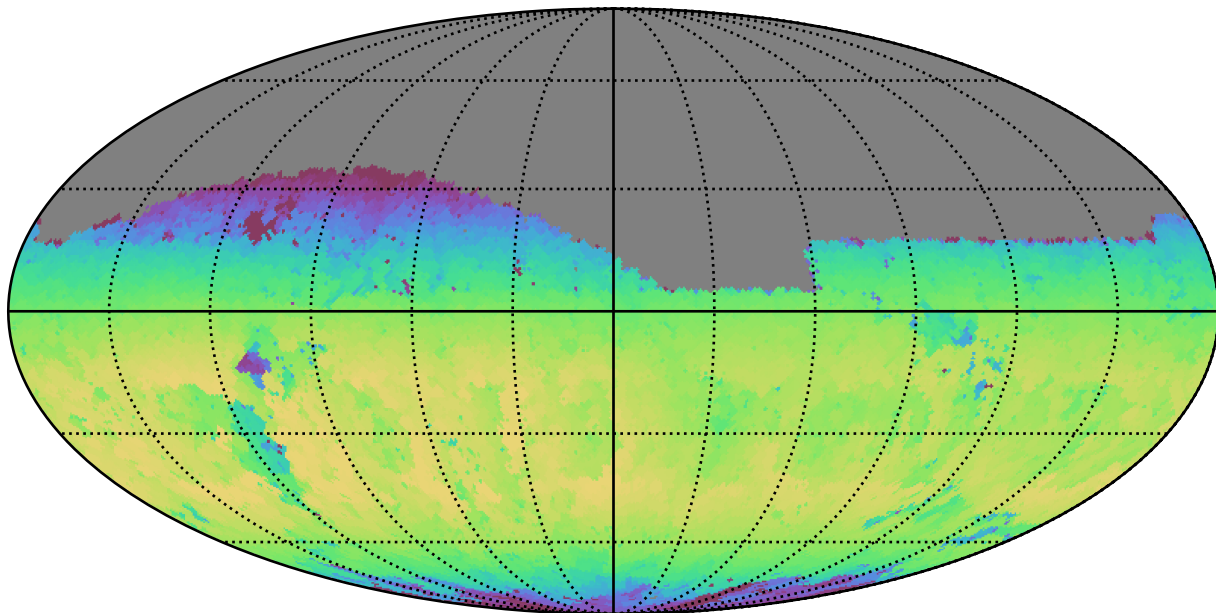
too_10_4v3.4_10yrs Yr 1 z band: Max skyBrightness
