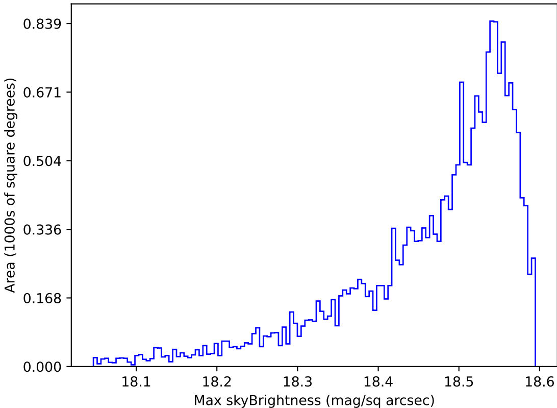
too_10_4v3.4_10yrs Yr 1 y band: Max skyBrightness
