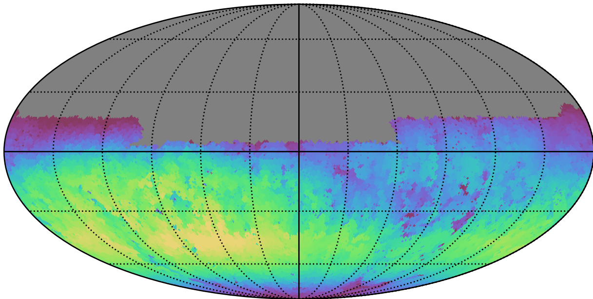
too_10_4v3.4_10yrs Yr 1 u band: Max skyBrightness
