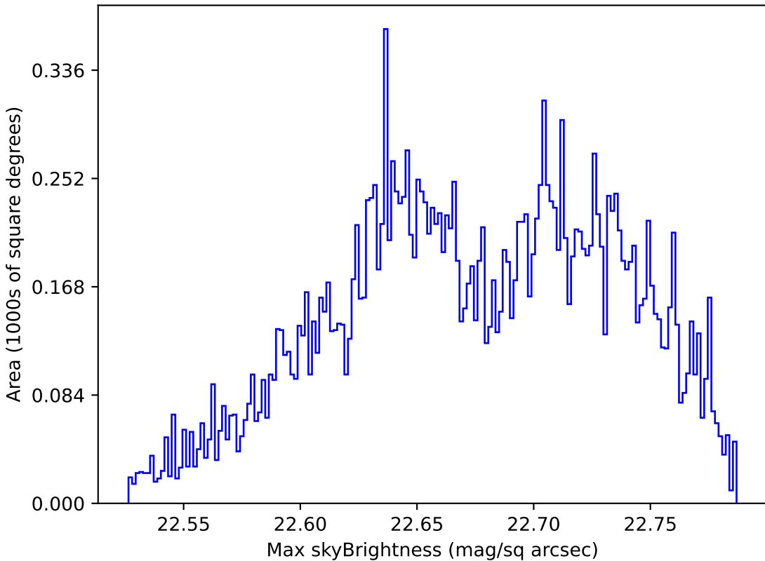
too_10_4v3.4_10yrs Yr 1 u band: Max skyBrightness
