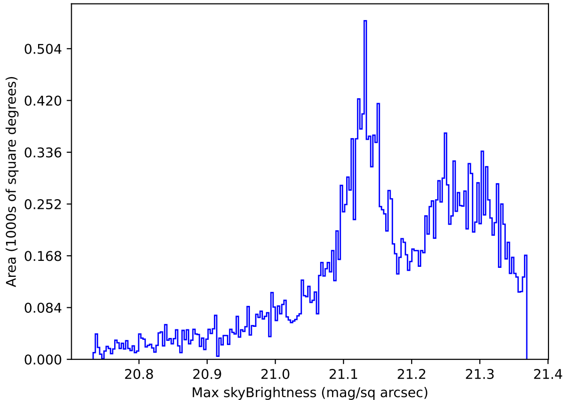
too_10_4v3.4_10yrs Yr 1 r band: Max skyBrightness
