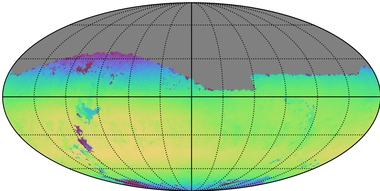
too_10_4v3.4_10yrs Yr 1 i band: Max skyBrightness
