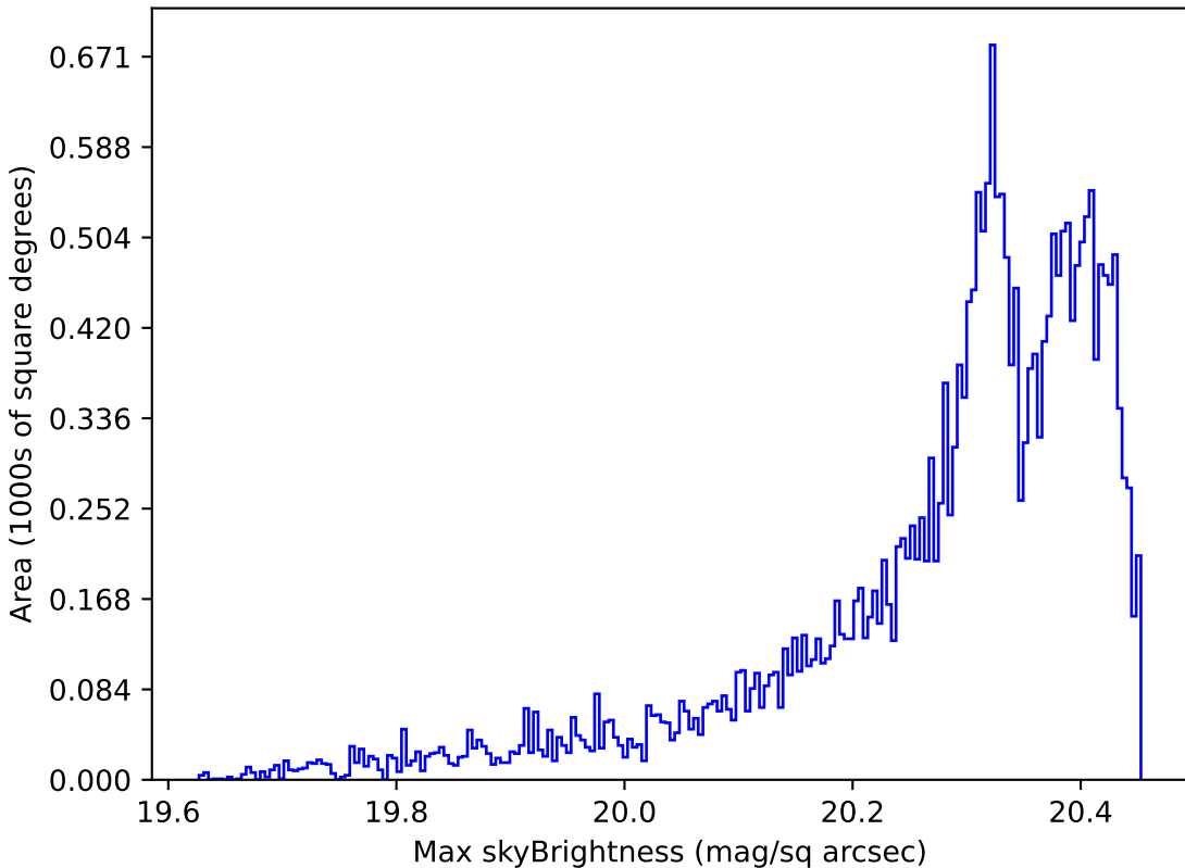
too_10_4v3.4_10yrs Yr 1 i band: Max skyBrightness
