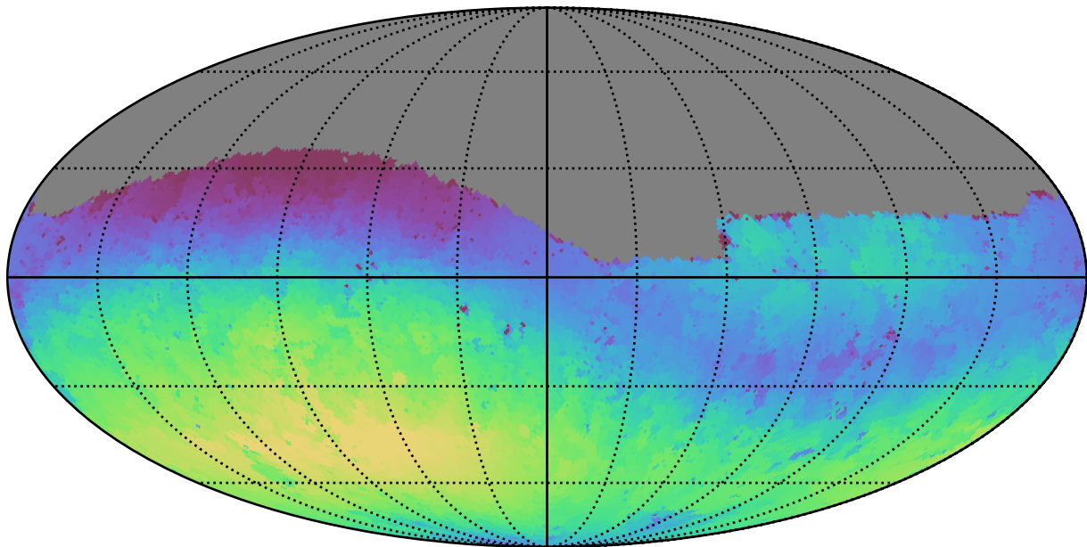
too_10_4v3.4_10yrs Yr 1 g band: Max skyBrightness
