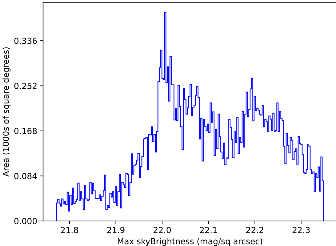
too_10_4v3.4_10yrs Yr 1 g band: Max skyBrightness
