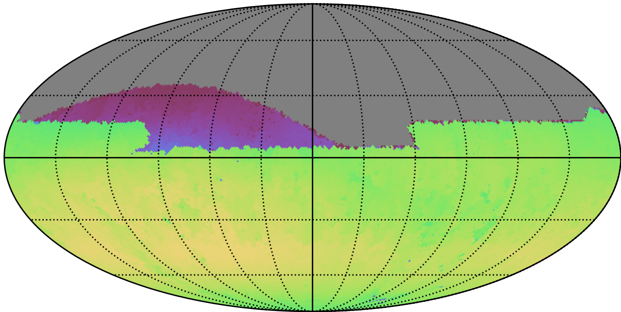
too_10_4v3.4_10yrs Yr 1 all bands: Max skyBrightness
