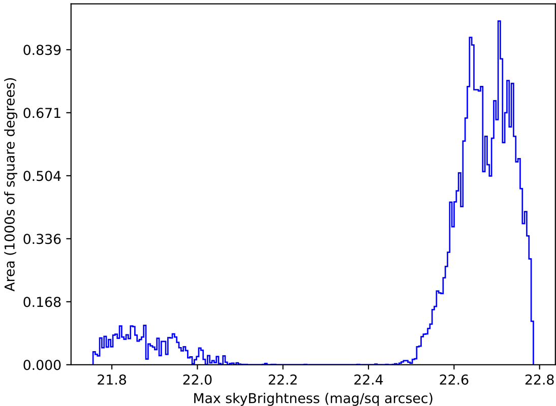
too_10_4v3.4_10yrs Yr 1 all bands: Max skyBrightness
