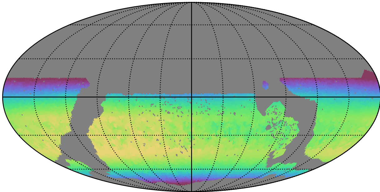
too_10_4v3.4_10yrs WFD z band: Max skyBrightness
