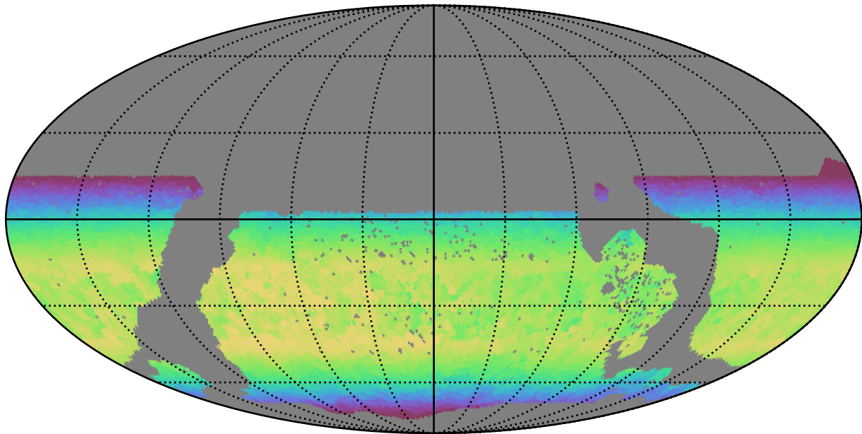
too_10_4v3.4_10yrs WFD y band: Max skyBrightness
