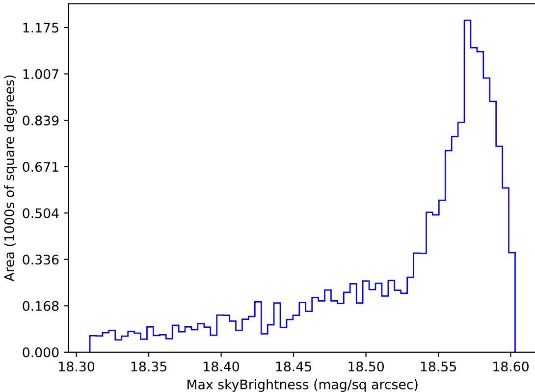
too_10_4v3.4_10yrs WFD y band: Max skyBrightness
