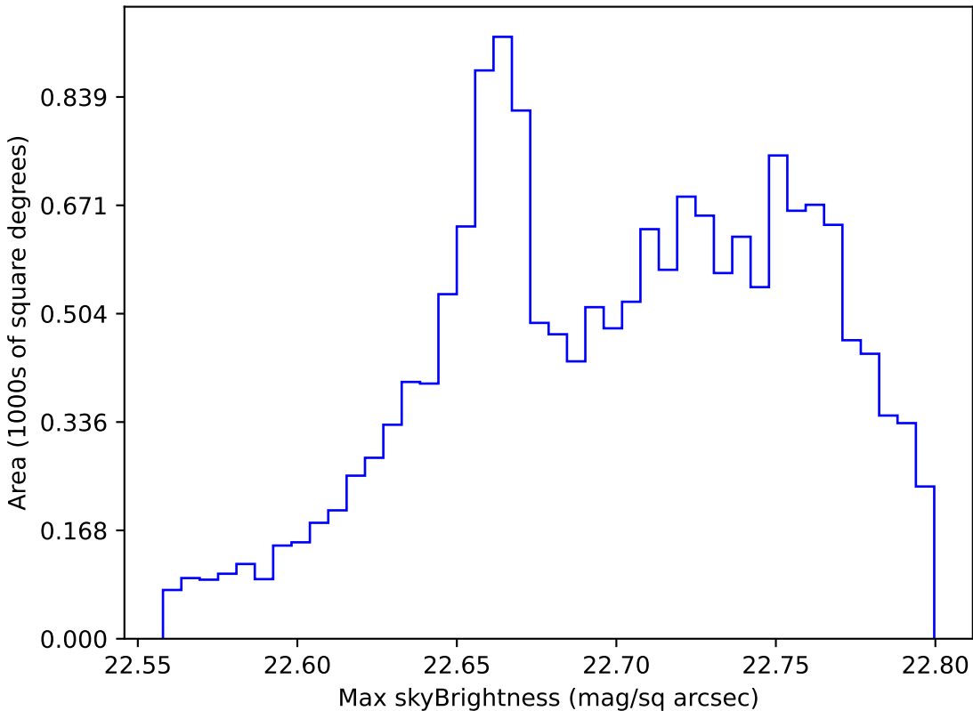
too_10_4v3.4_10yrs WFD u band: Max skyBrightness
