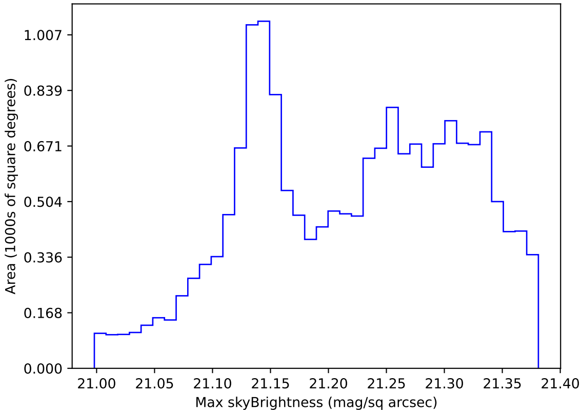
too_10_4v3.4_10yrs WFD r band: Max skyBrightness
