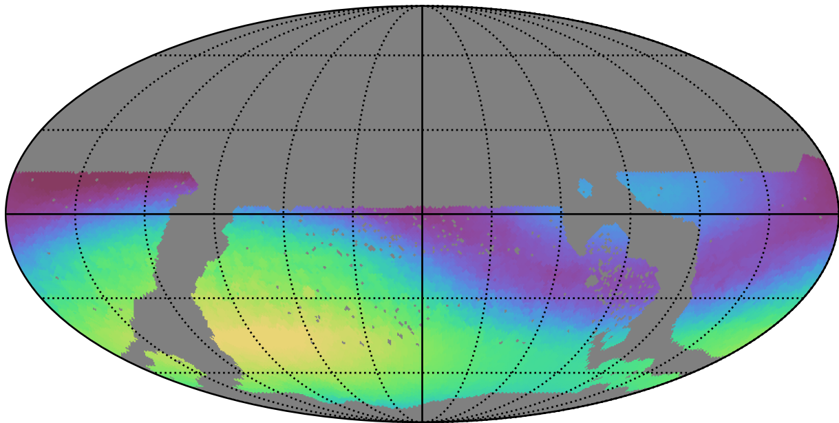
too_10_4v3.4_10yrs WFD g band: Max skyBrightness
