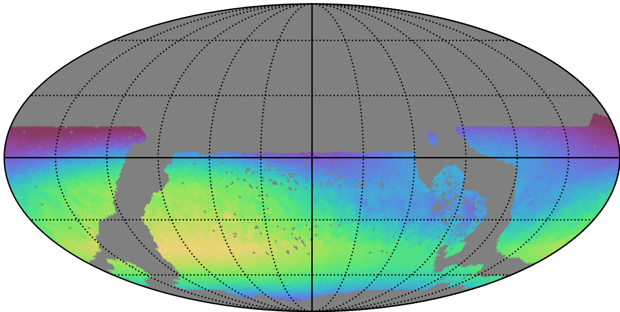
too_10_4v3.4_10yrs WFD all bands: Max skyBrightness
