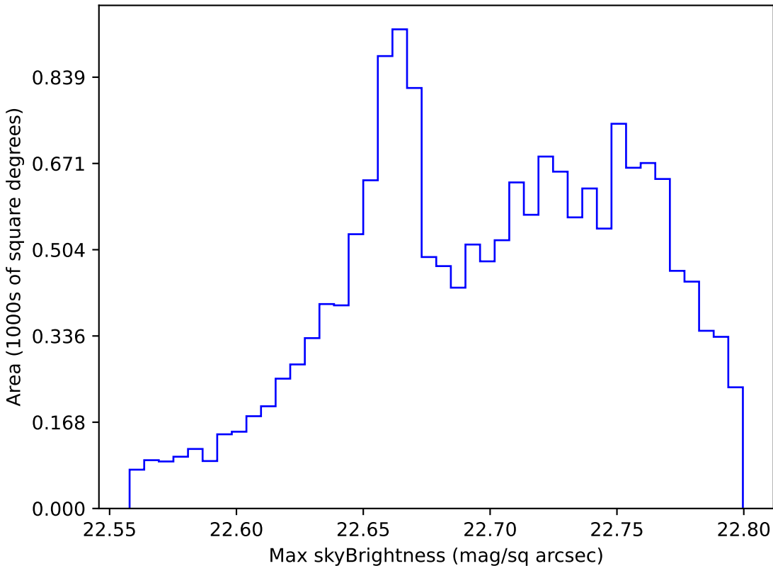
too_10_4v3.4_10yrs WFD all bands: Max skyBrightness
