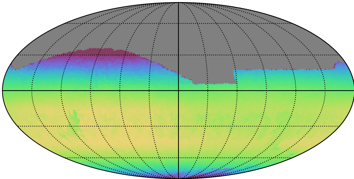
too_10_4v3.4_10yrs All sky z band: Max skyBrightness
