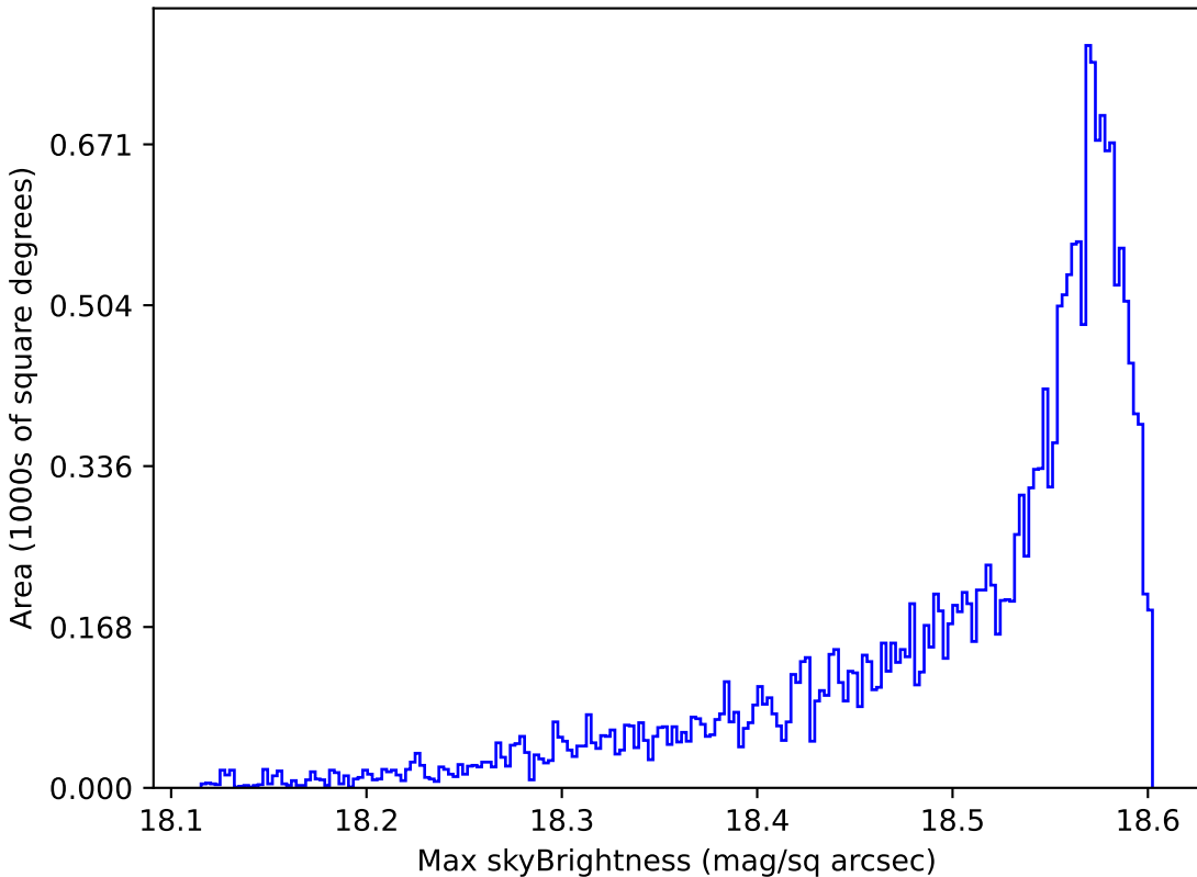
too_10_4v3.4_10yrs All sky y band: Max skyBrightness
