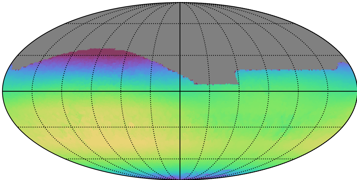
too_10_4v3.4_10yrs All sky i band: Max skyBrightness
